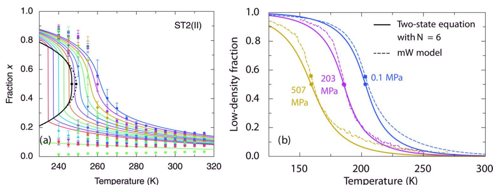
Figure 8. Low-density fraction from simulations of water-like models, and the predictions from the two-state thermodynamics (Reproduced with permission from ref 163 . Copyright 2014 AIP Publishing LLC): (a) ST2(II) (denoted ST2b in Table 1), a version of the ST2 model. 163 Fraction x is the low-density fraction. Symbols are simulation data. Solid curves are theoretical predictions. Dashed curve is a mean-field approximation. (b) mW model. Reproduced with permission from ref 136 . Copyright 2013 AIP Publishing LLC. Solid curves are theoretical predictions which include clustering of water molecules with average aggregation number N = 6 .
