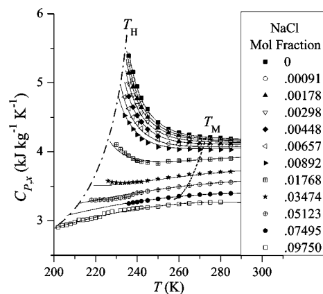
Figure 25. Suppression of the anomaly of the heat capacity in aqueous solutions of sodium chloride (Reproduced with permission from ref 159 . Copyright 2014 AIP Publishing LLC). Symbols: experimental data of Archer and Carter. 372,373 Solid curves: predictions based on two-state thermodynamics. 159 Dashed curve shows the positions of the melting temperatures. Dashed-dotted curve shows the temperatures of homogeneous ice formation.
