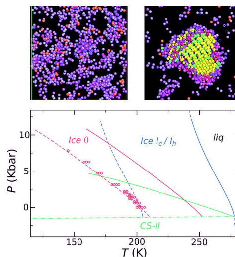
Figure 20. (Top) Snapshot of two configurations with the birth of a small crystalline nucleus (left) and a section of a nucleus of critical size (right). The color code is yellow for ice I h , green for ice I h , and magenta for ice 0. (Bottom) P – T phase diagram of mW water. Continuous lines indicate coexistence between the liquid phase and different crystal structures: ice I h / I c (blue), ice 0 (red), and clathrate CS-II (green). Dashed lines indicate constant chemical potential differences between the liquid and ice I h / I c ( \beta\Delta\mu = -0.721 , in blue) and the liquid and ice 0 ( \beta\Delta\mu = -0.365 , in red). The green dashed-dotted line is the I c /CS-II coexistence line. Red open circles indicate state points where homogeneous nucleation is observed in simulations. Adapted from ref 242. Copyright 2014 Macmillan Publishers Limited.
